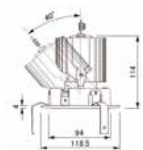
NPD-U100-21/30-NW[3000K]
