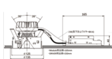
NPD-U125-15/27D-NW[2700K]
