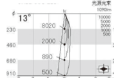
NPD-U125-15/27D-NW[2700K]
